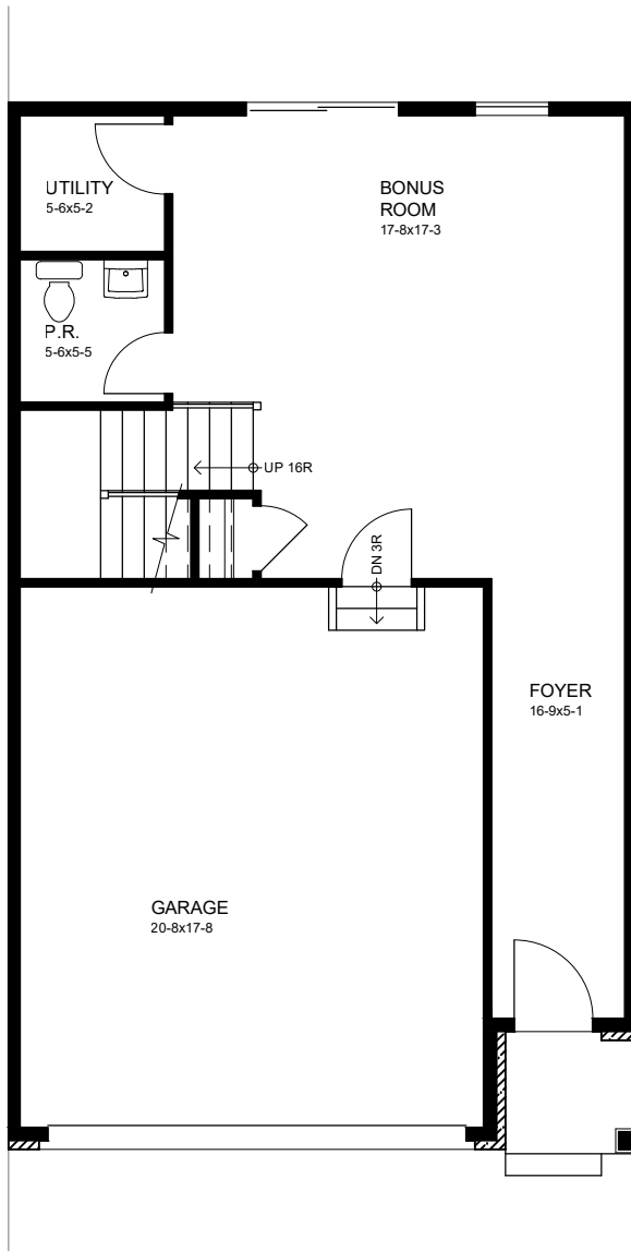
TOWNHOUSE MIDDLE UNIT FIRST FLOOR PLAN
