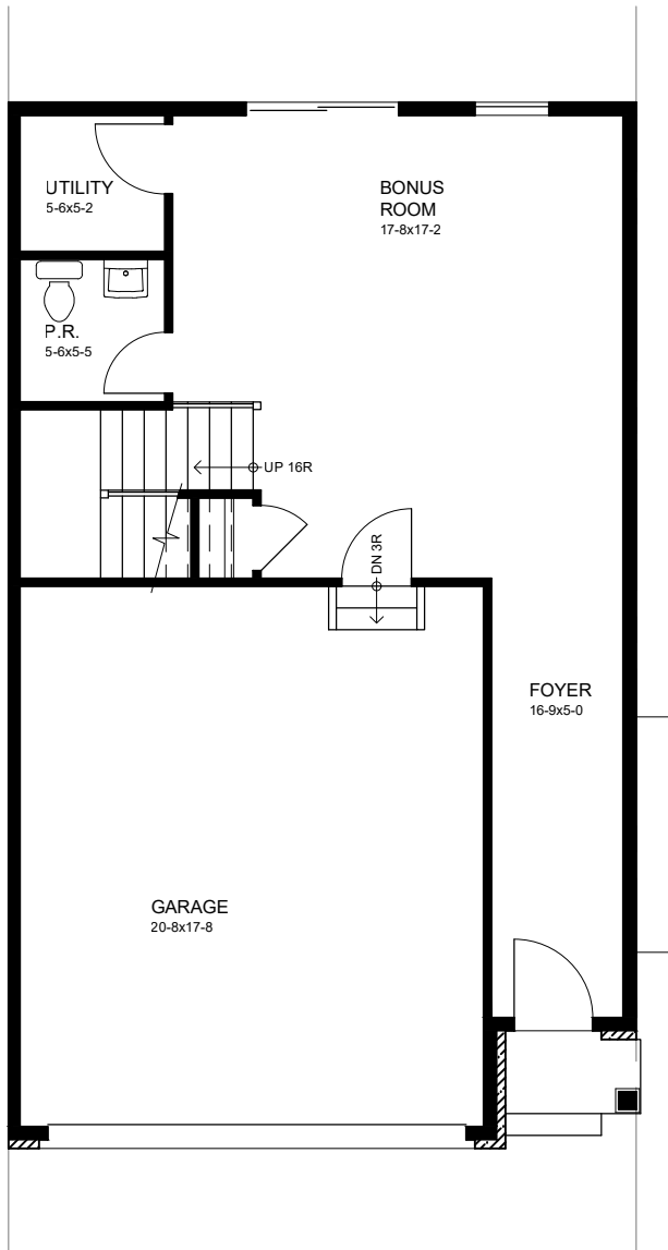
TOWNHOUSE END UNIT FIRST FLOOR PLAN
