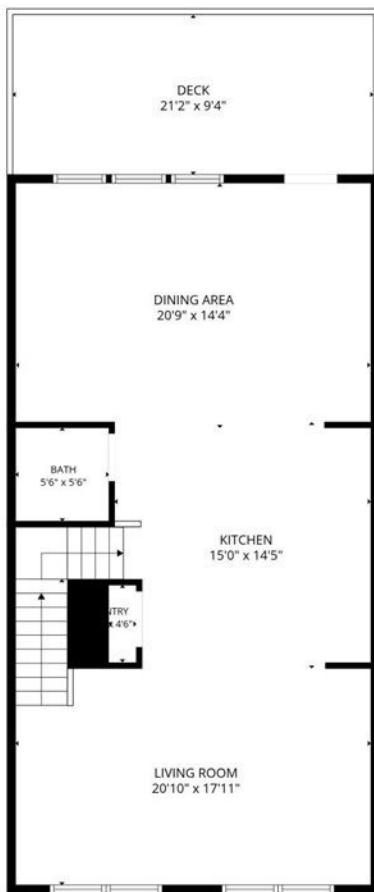
2nd floor
